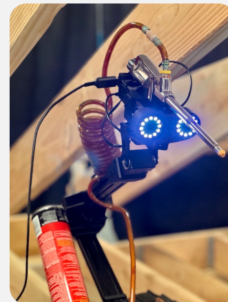
5-DoF Foam Spray Turret
