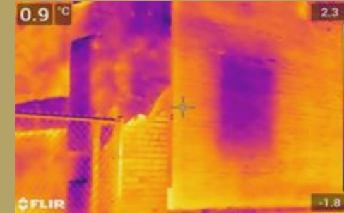
Building Envelope Thermography to Diagnose Thermal Anomalies
