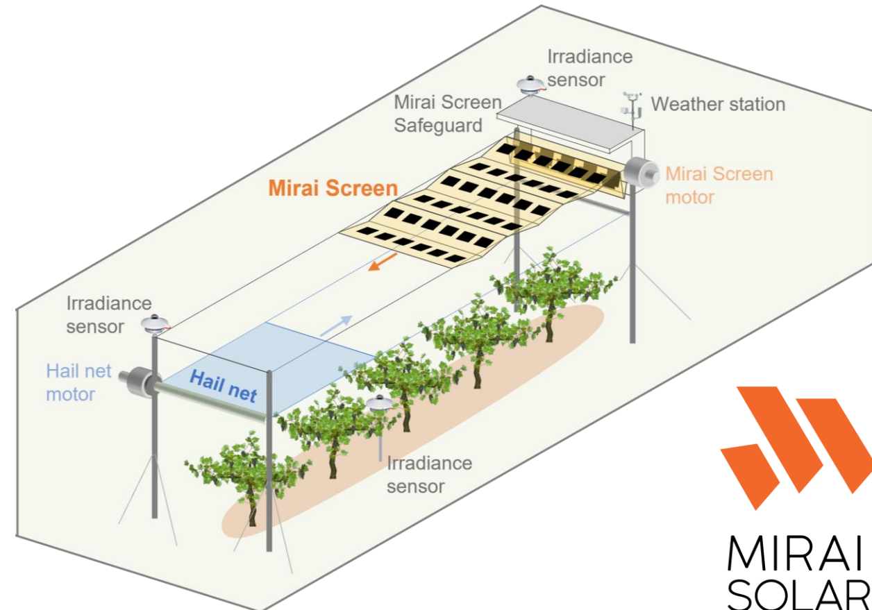
Prototype of Mirai Screen with half-cut bifacial cells
