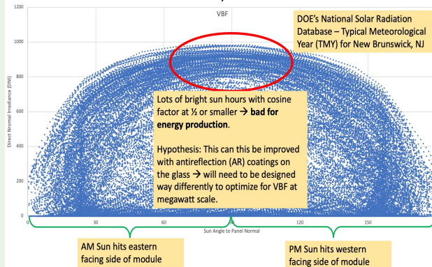
Vertical Bifacial – Full Year, 5-Minute Intervals
