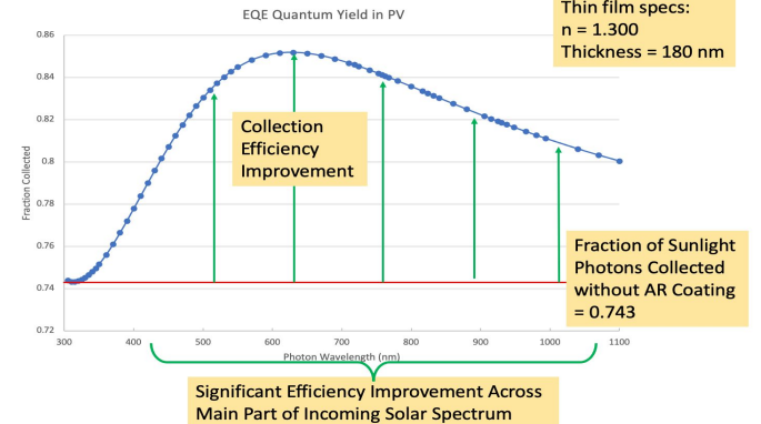
Solar Active Photon Fraction at 75° Oblique Incidence
