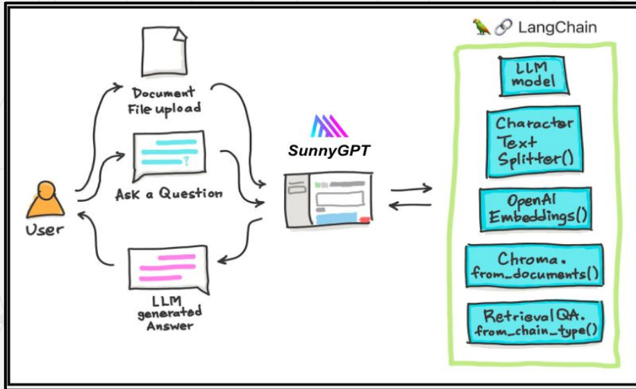
Figure 1. Sunny GPT chatbot tool interaction with the user and the LangChain solar database plugin.
