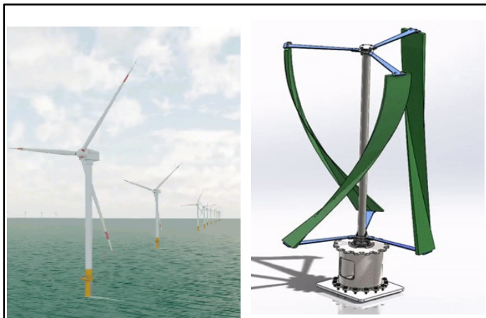
Horizontal axis (left, credit: vmts) and Vertical Axis (right, credit: Fasiai, 2021) Wind Turbines for Wind Energy Harvesting
