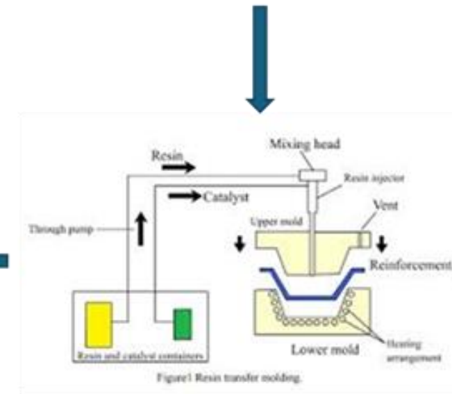
Resin Transfer Molding process
