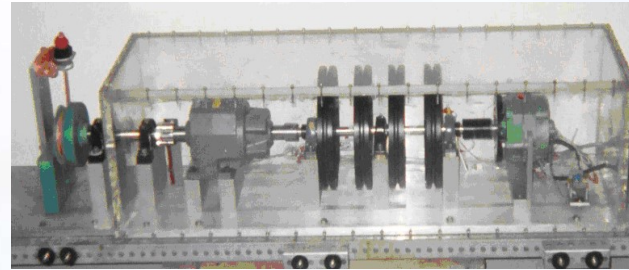
Pressurized Housing
