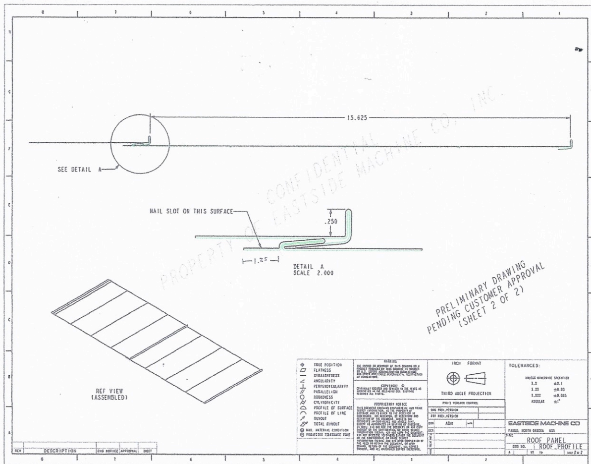
CAD representation of our patent pending panel.
