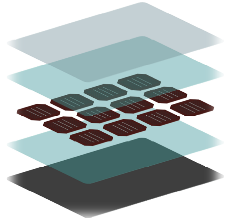
Perovskite solar cell layers
